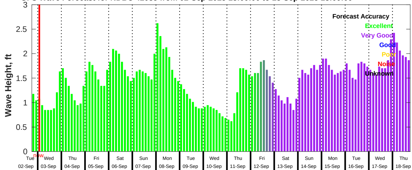
GFS Wave Forecast for NDBC 42035 from 02-Sep-2025 18:00:00 to 18-Sep-2025 18:00:00
