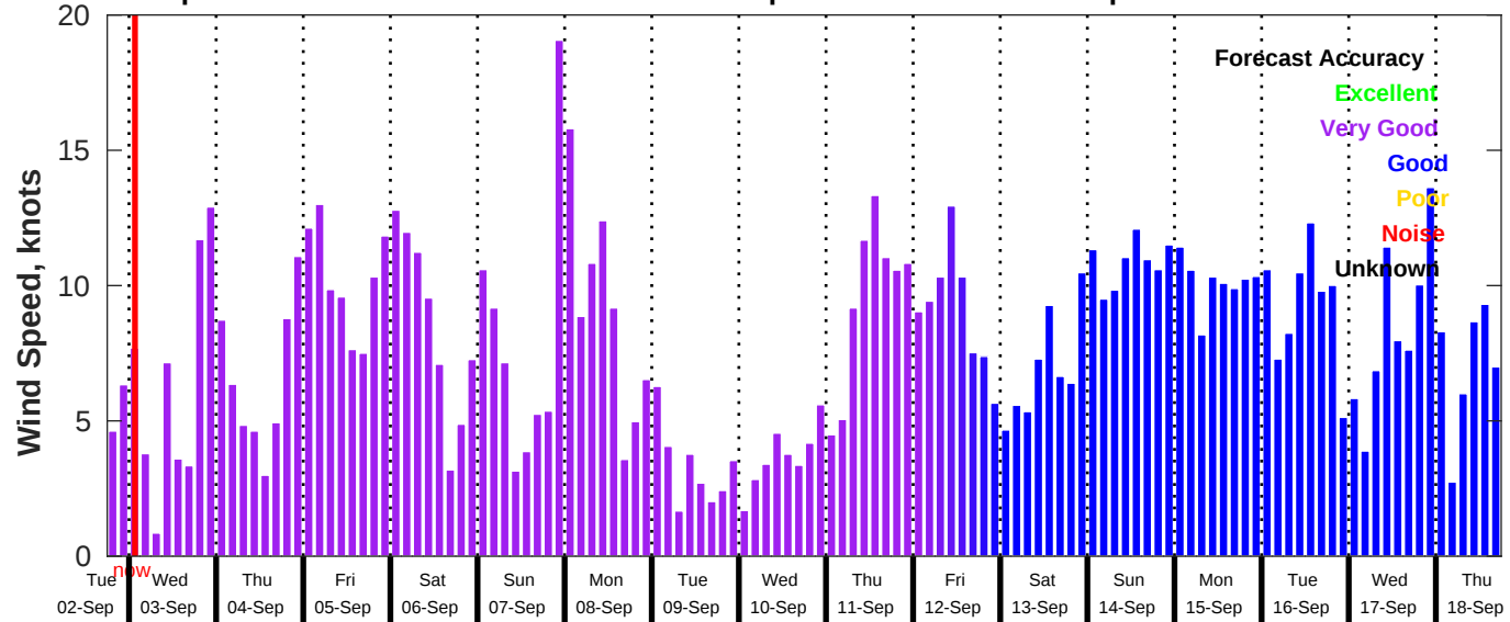
GFS Wind Speed Forecast for NDBC 42035 from 02-Sep-2025 18:00:00 to 18-Sep-2025 18:00:00
