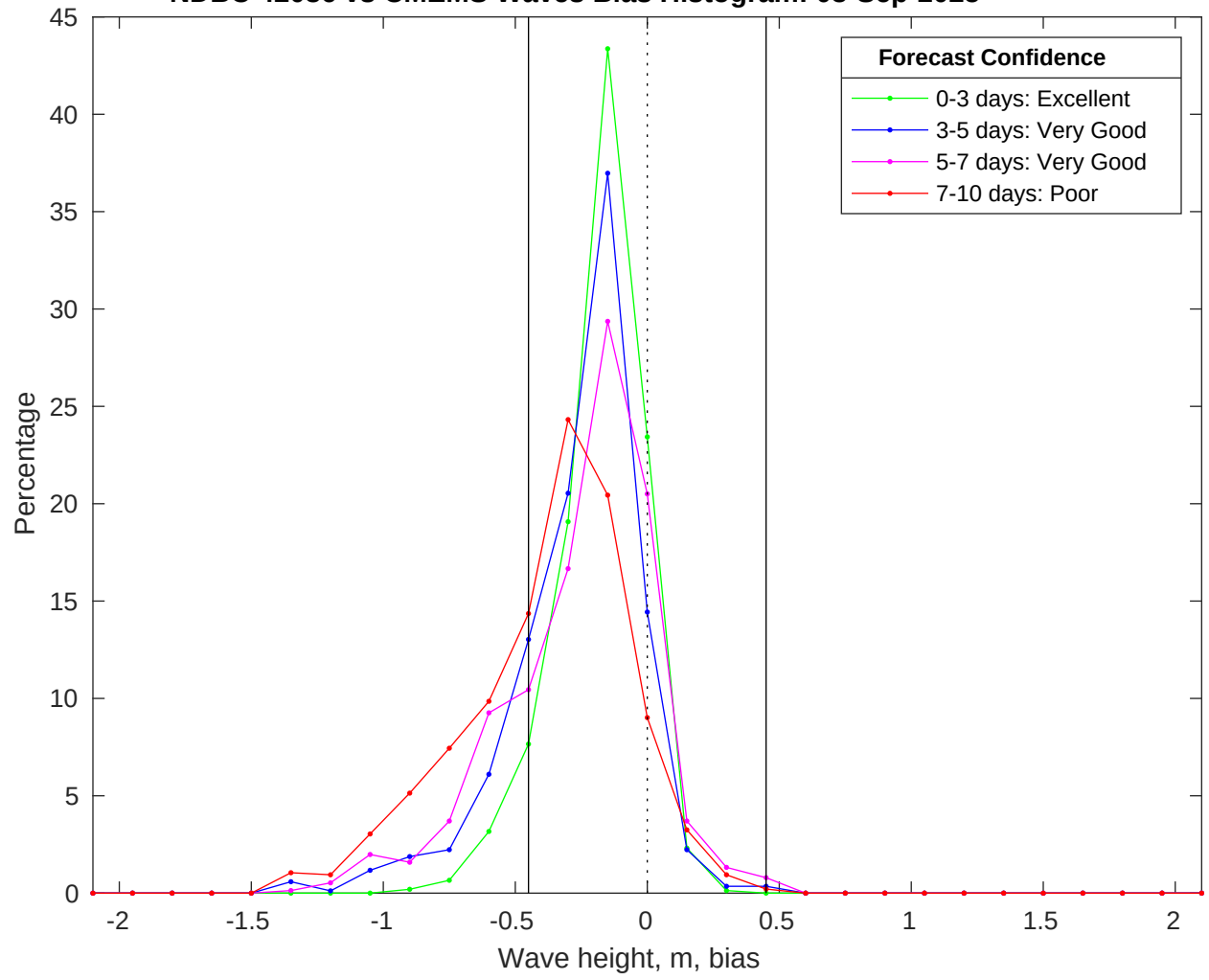
NDBC 42036 vs CMEMS Waves Bias Histogram: 03-Sep-2025
