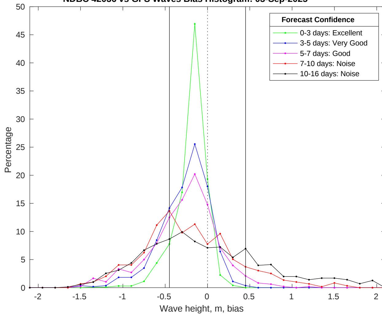
NDBC 42036 vs GFS Waves Bias Histogram: 03-Sep-2025
