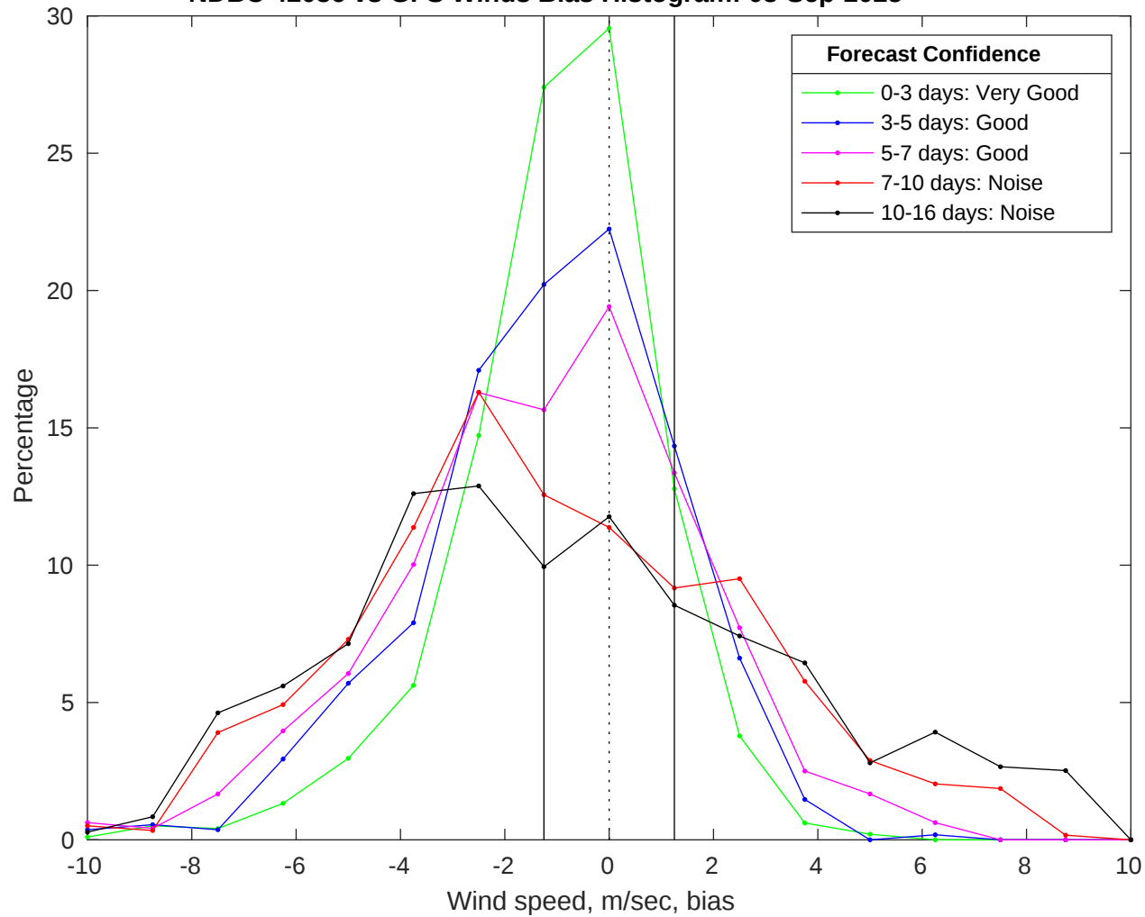
NDBC 42036 vs GFS Winds Bias Histogram: 03-Sep-2025
