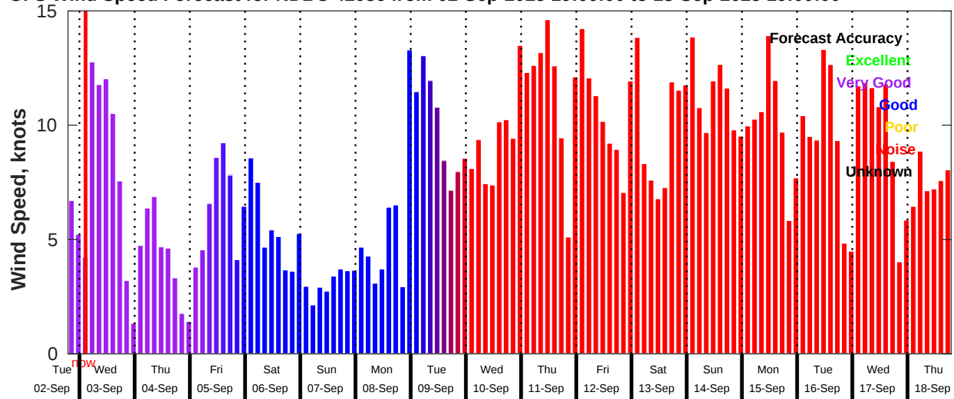
GFS Wind Speed Forecast for NDBC 42036 from 02-Sep-2025 19:00:00 to 18-Sep-2025 19:00:00
