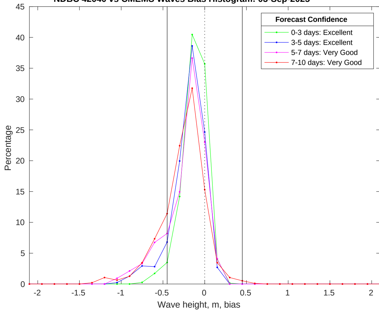
NDBC 42040 vs CMEMS Waves Bias Histogram: 03-Sep-2025
