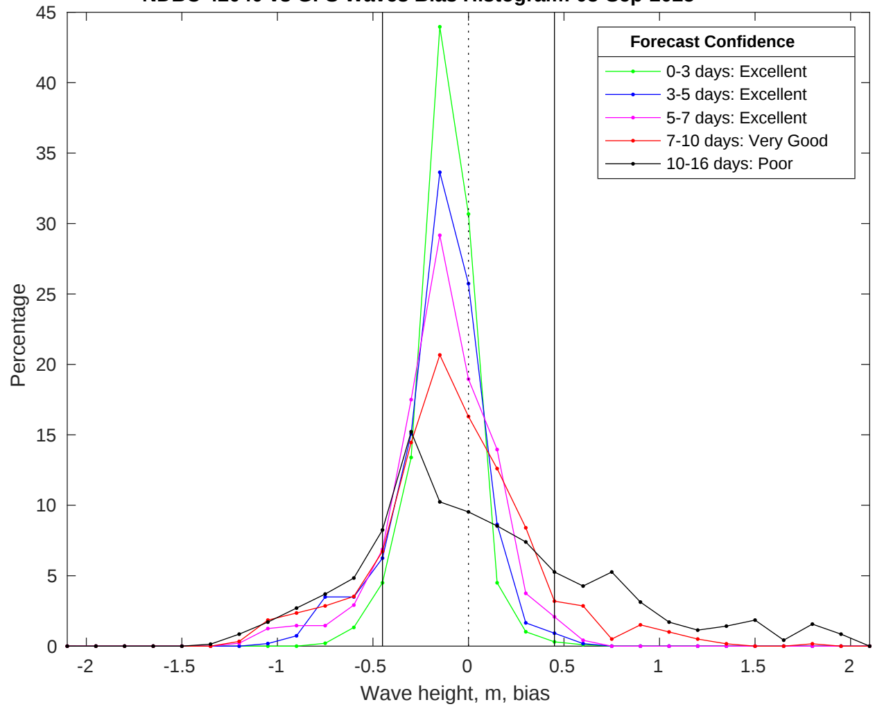
NDBC 42040 vs GFS Waves Bias Histogram: 03-Sep-2025
