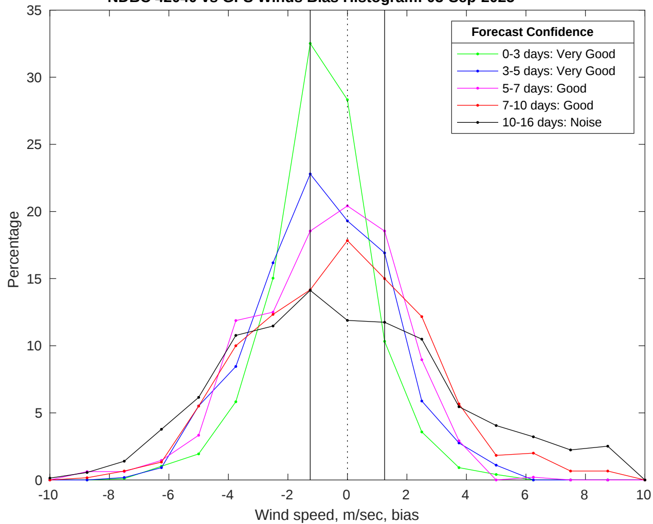
NDBC 42040 vs GFS Winds Bias Histogram: 03-Sep-2025
