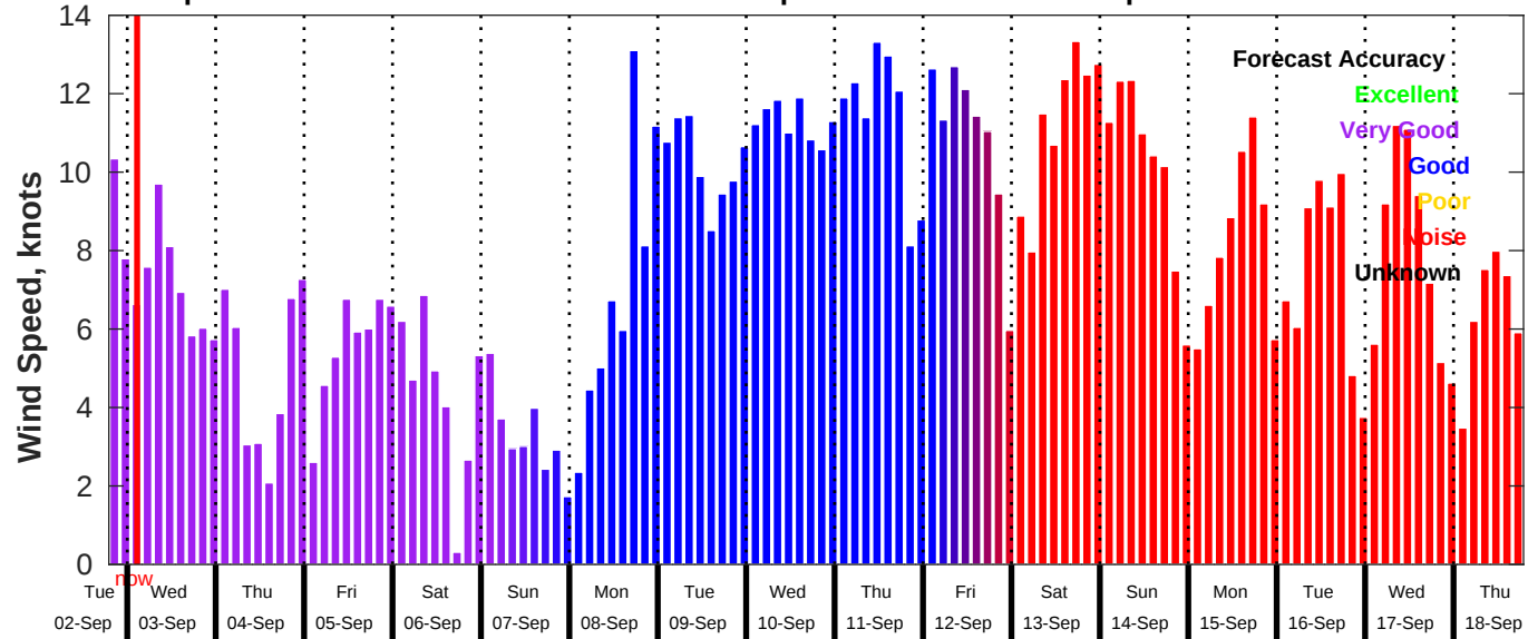
GFS Wind Speed Forecast for NDBC 42040 from 02-Sep-2025 19:00:00 to 18-Sep-2025 19:00:00
