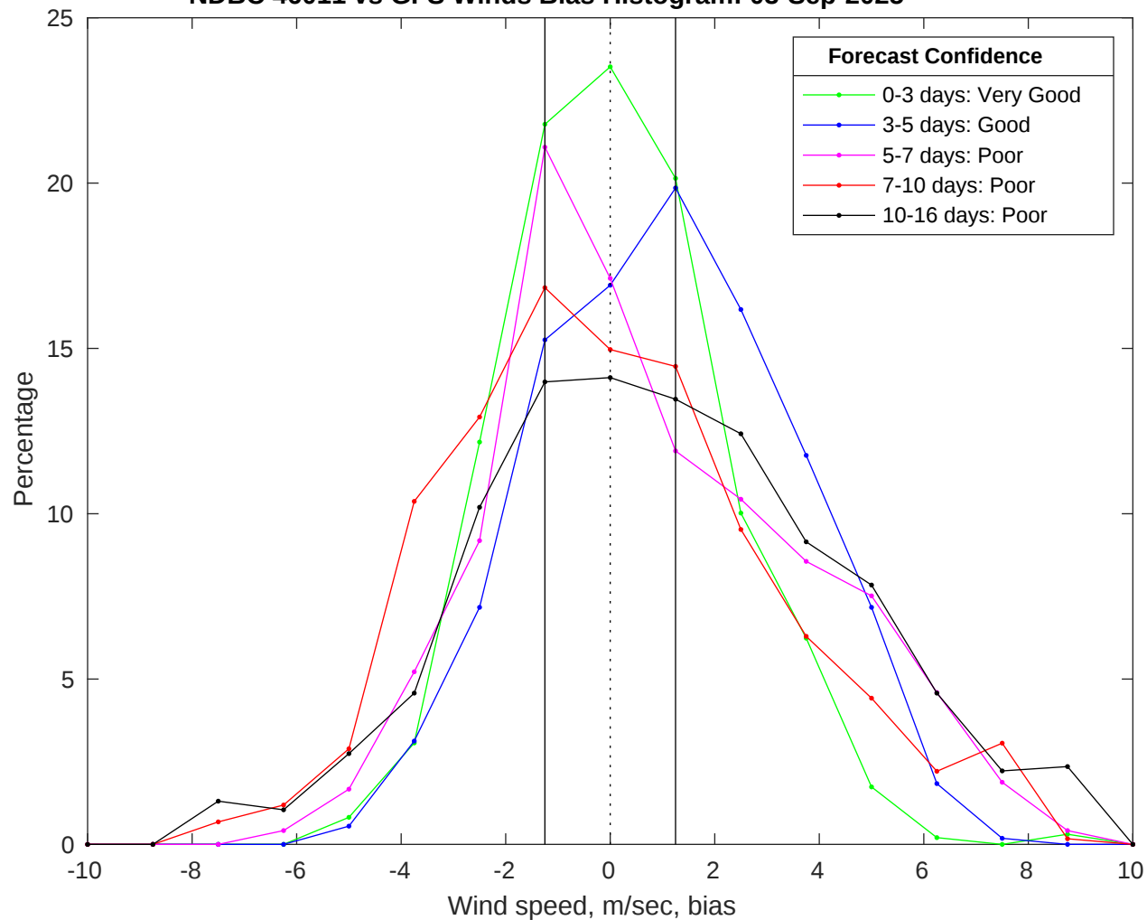
NDBC 46011 vs GFS Winds Bias Histogram: 03-Sep-2025
