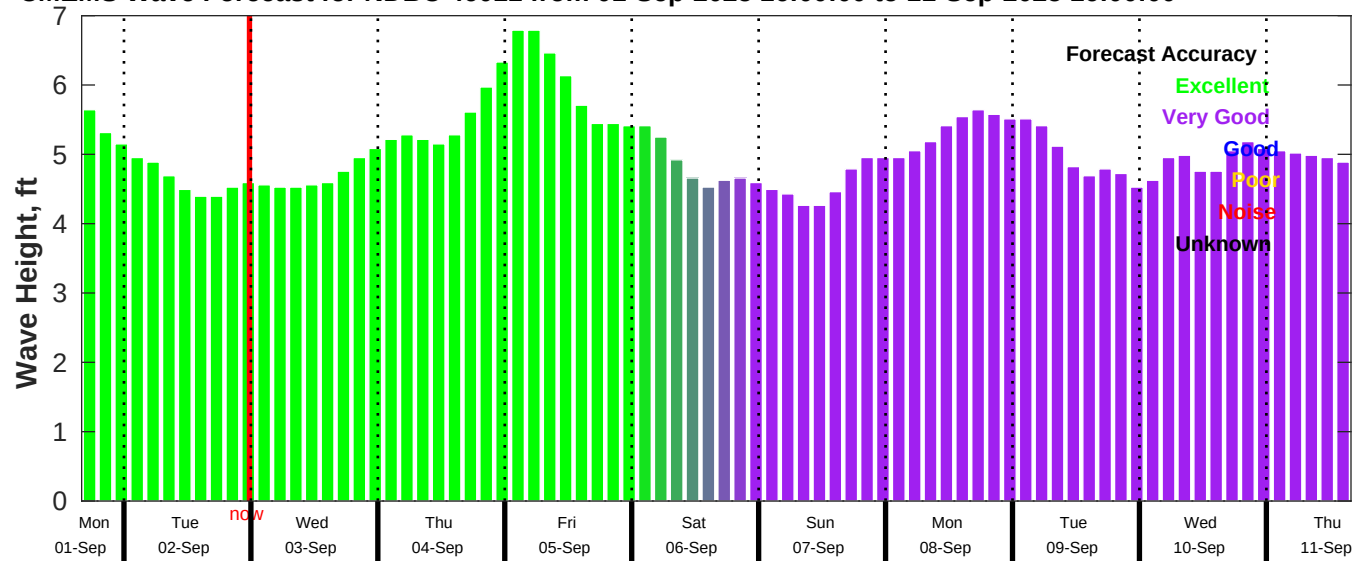
CMEMS Wave Forecast for NDBC 46011 from 01-Sep-2025 16:00:00 to 11-Sep-2025 16:00:00
