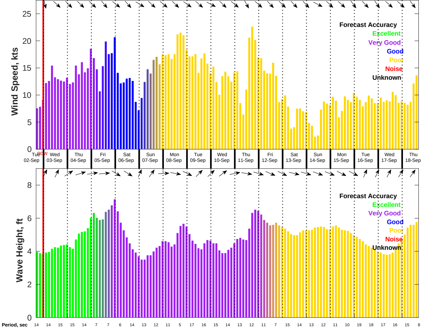
Wind & Wave Forecast for NDBC 46011 from 02-Sep-2025 16:00:00 to 18-Sep-2025 16:00:00
