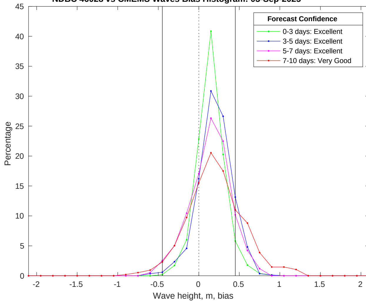
NDBC 46028 vs CMEMS Waves Bias Histogram: 03-Sep-2025
