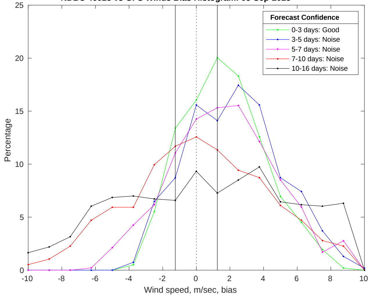
NDBC 46028 vs GFS Winds Bias Histogram: 03-Sep-2025
