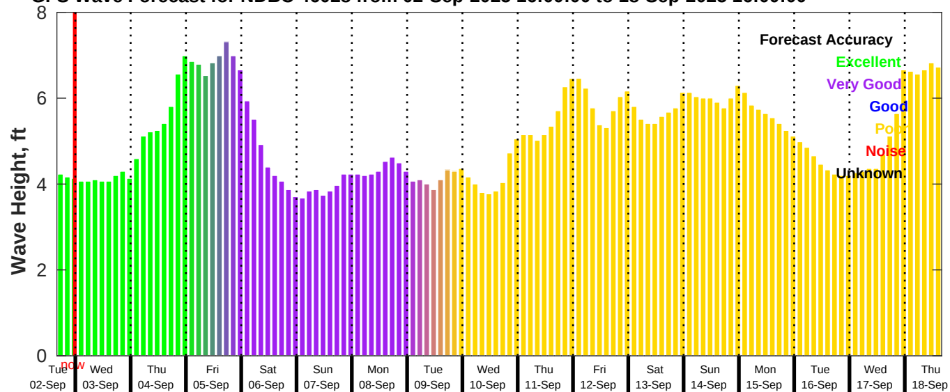
GFS Wave Forecast for NDBC 46028 from 02-Sep-2025 16:00:00 to 18-Sep-2025 16:00:00
