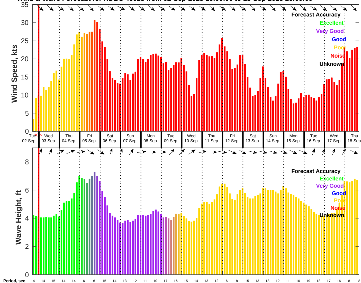
Wind & Wave Forecast for NDBC 46028 from 02-Sep-2025 16:00:00 to 18-Sep-2025 16:00:00
