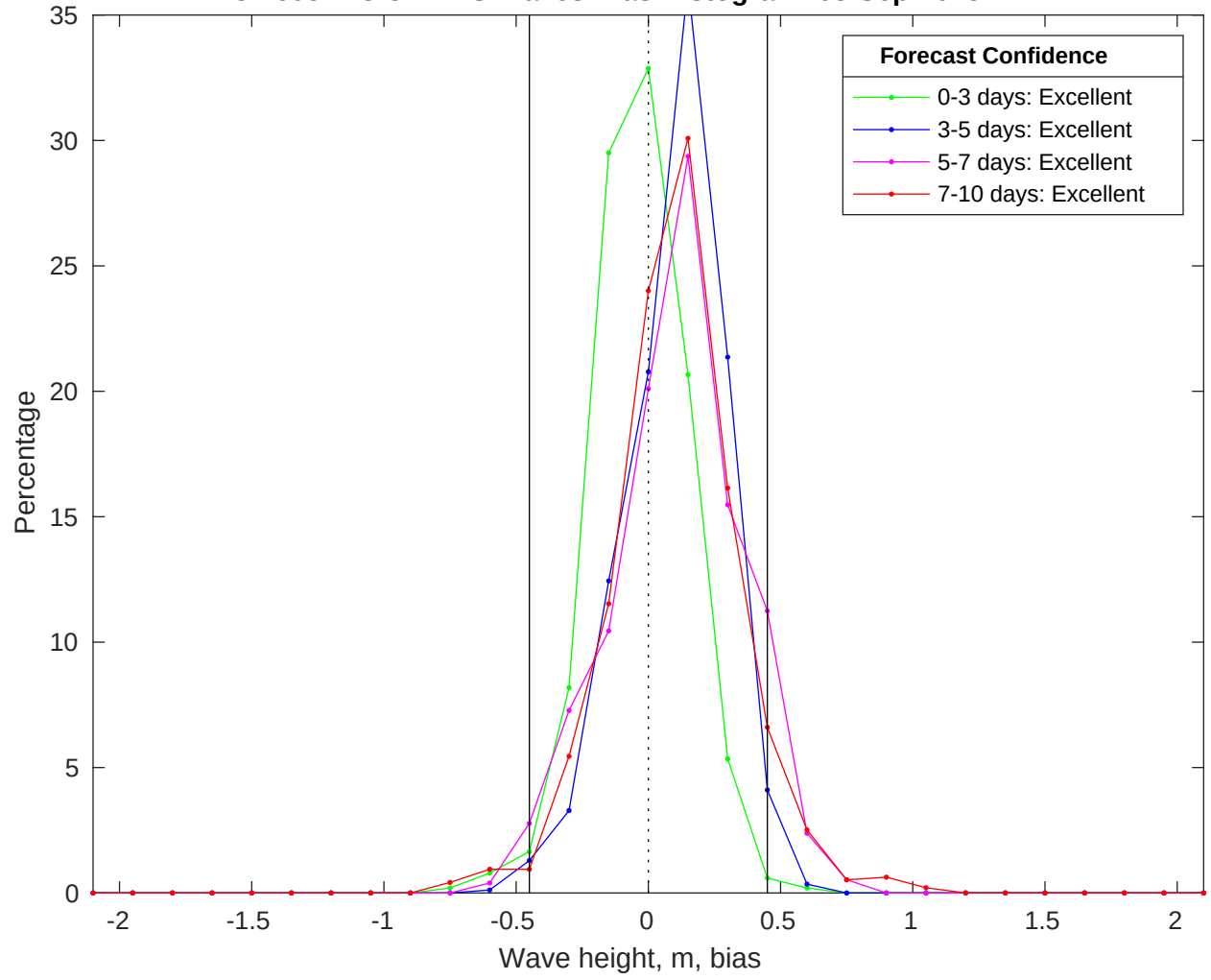
NDBC 46054 vs CMEMS Waves Bias Histogram: 03-Sep-2025
