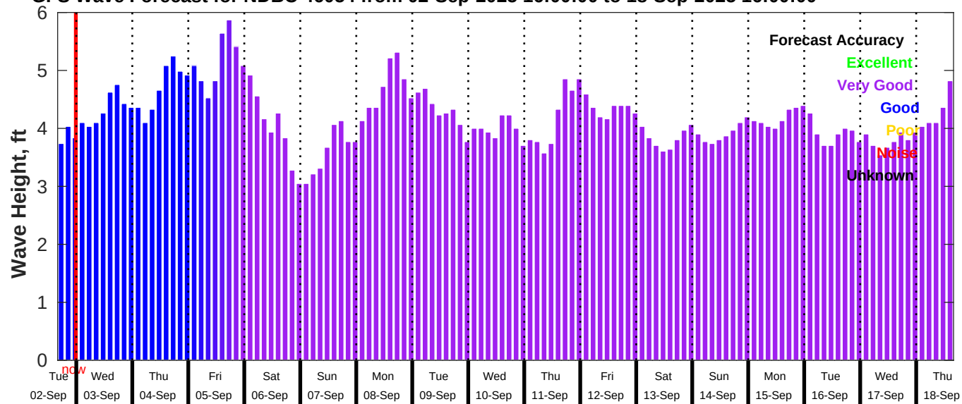
GFS Wave Forecast for NDBC 46054 from 02-Sep-2025 16:00:00 to 18-Sep-2025 16:00:00
