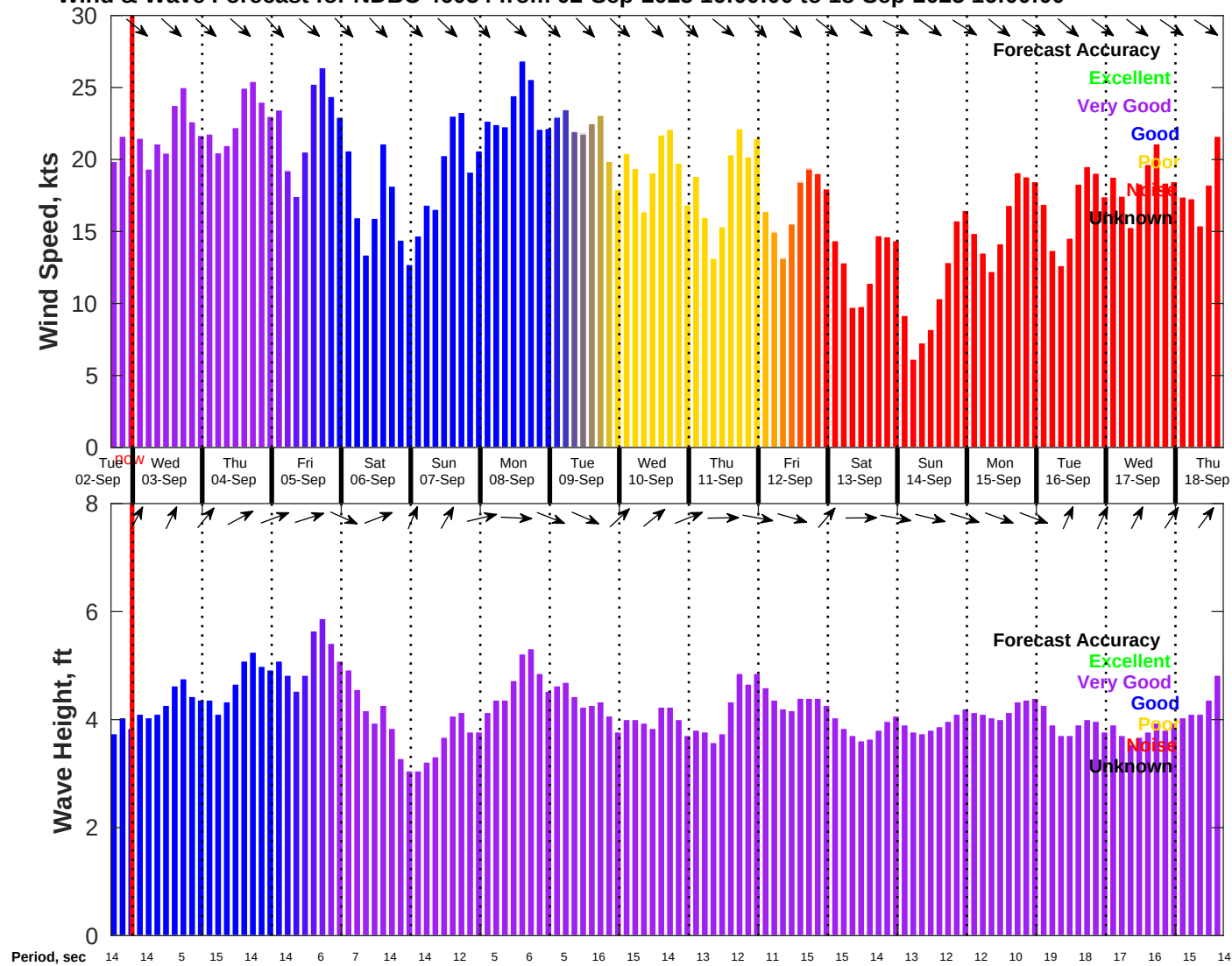
Wind & Wave Forecast for NDBC 46054 from 02-Sep-2025 16:00:00 to 18-Sep-2025 16:00:00
