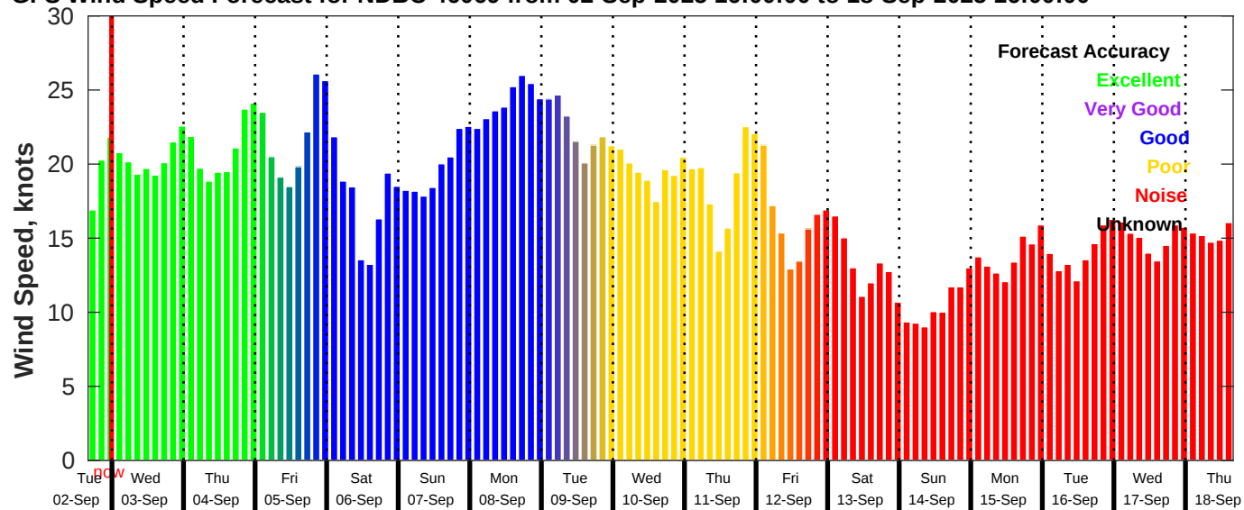
GFS Wind Speed Forecast for NDBC 46069 from 02-Sep-2025 16:00:00 to 18-Sep-2025 16:00:00
