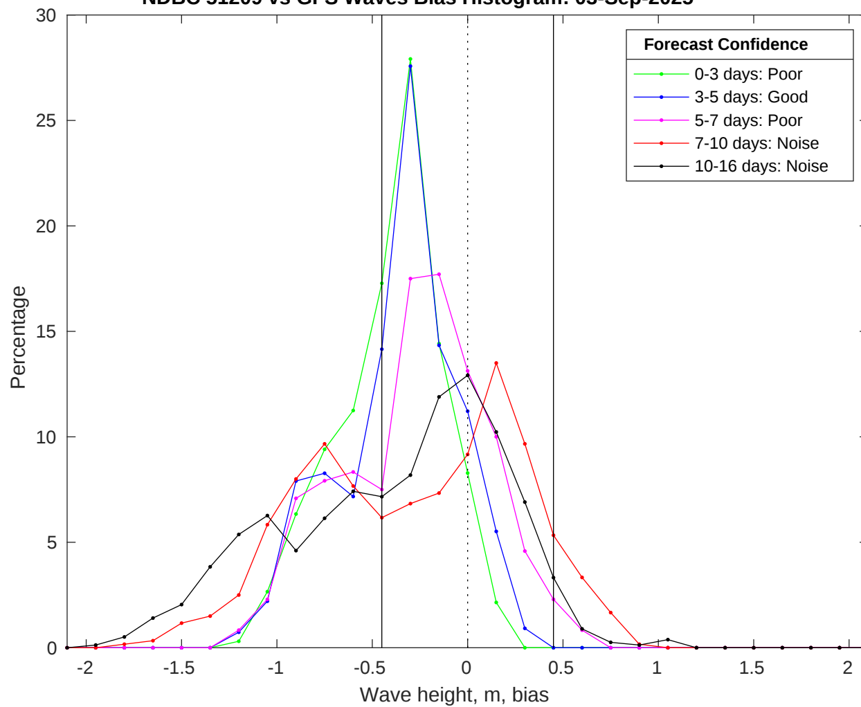
NDBC 51209 vs GFS Waves Bias Histogram: 03-Sep-2025
