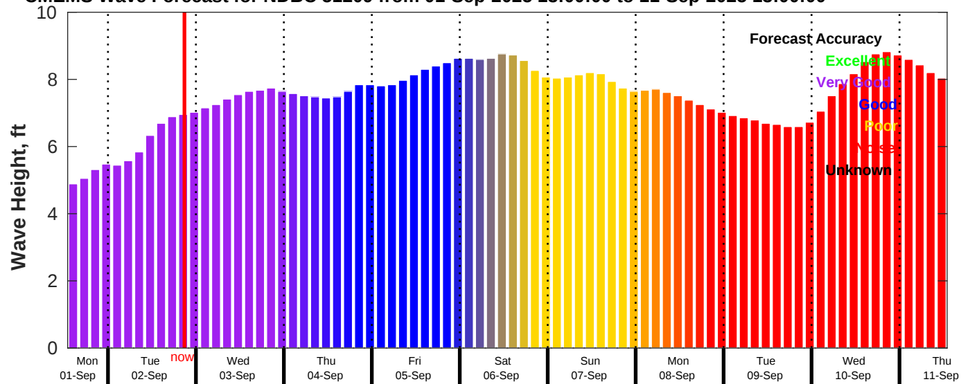
CMEMS Wave Forecast for NDBC 51209 from 01-Sep-2025 13:00:00 to 11-Sep-2025 13:00:00
