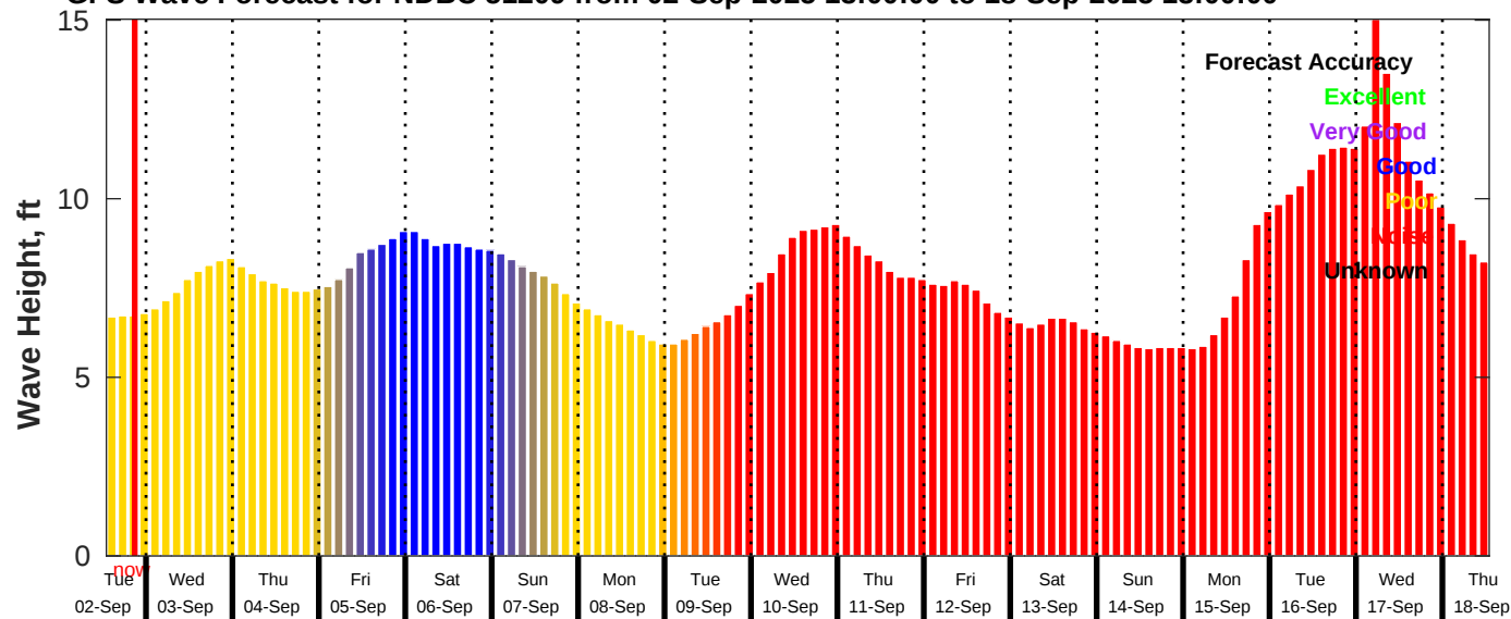
GFS Wave Forecast for NDBC 51209 from 02-Sep-2025 13:00:00 to 18-Sep-2025 13:00:00
