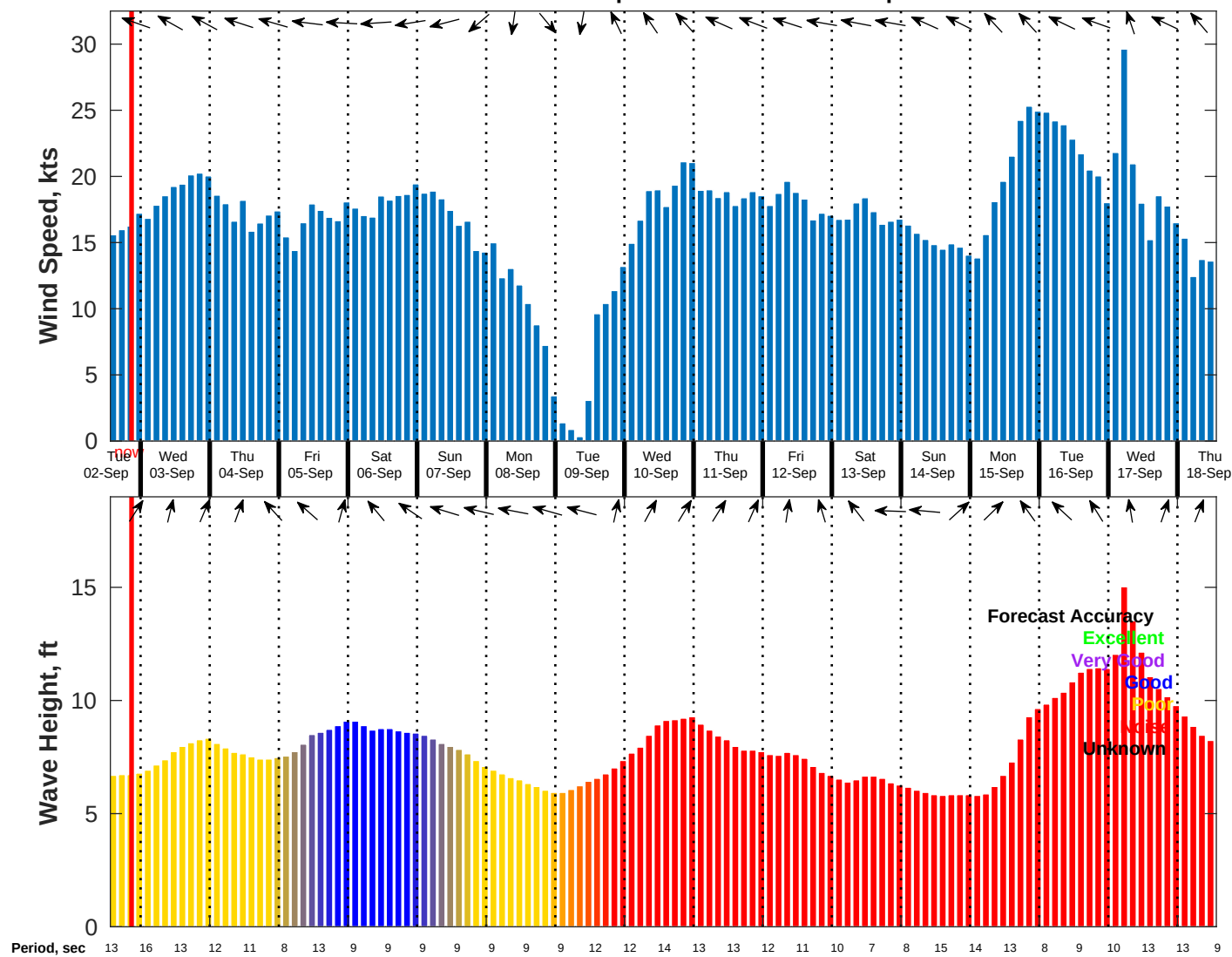
Wind & Wave Forecast for NDBC 51209 from 02-Sep-2025 13:00:00 to 18-Sep-2025 13:00:00
