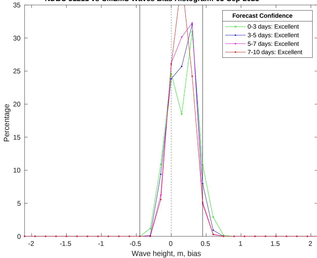
NDBC 51211 vs CMEMS Waves Bias Histogram: 03-Sep-2025
