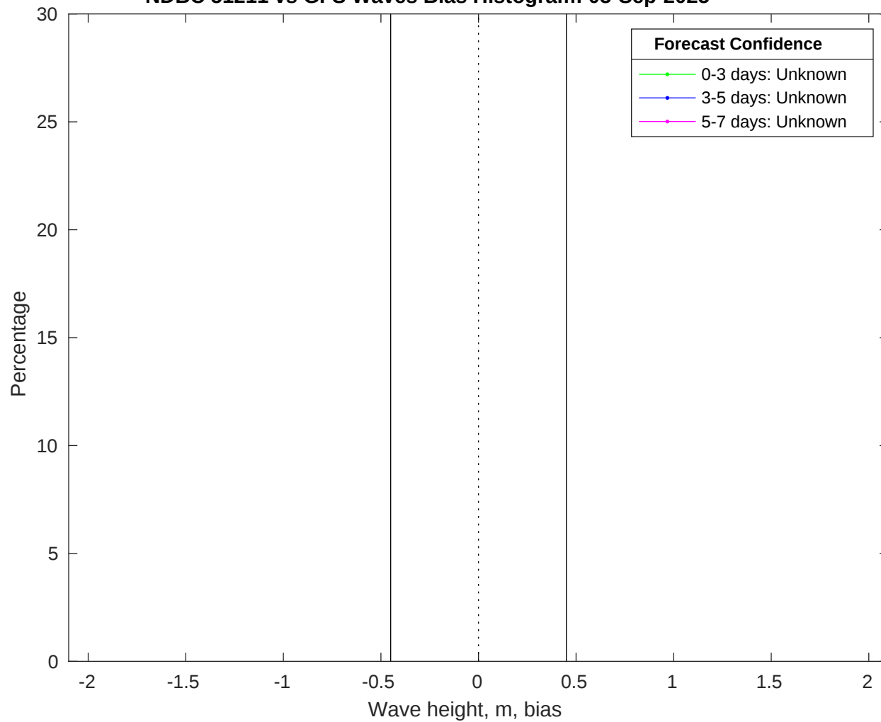
NDBC 51211 vs GFS Waves Bias Histogram: 03-Sep-2025
