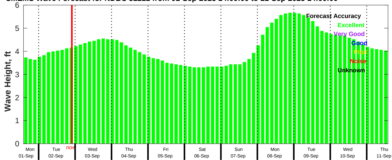
CMEMS Wave Forecast for NDBC 51211 from 01-Sep-2025 14:00:00 to 11-Sep-2025 14:00:00
