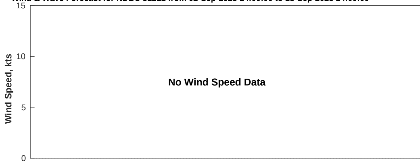
Wind & Wave Forecast for NDBC 51211 from 02-Sep-2025 14:00:00 to 18-Sep-2025 14:00:00
