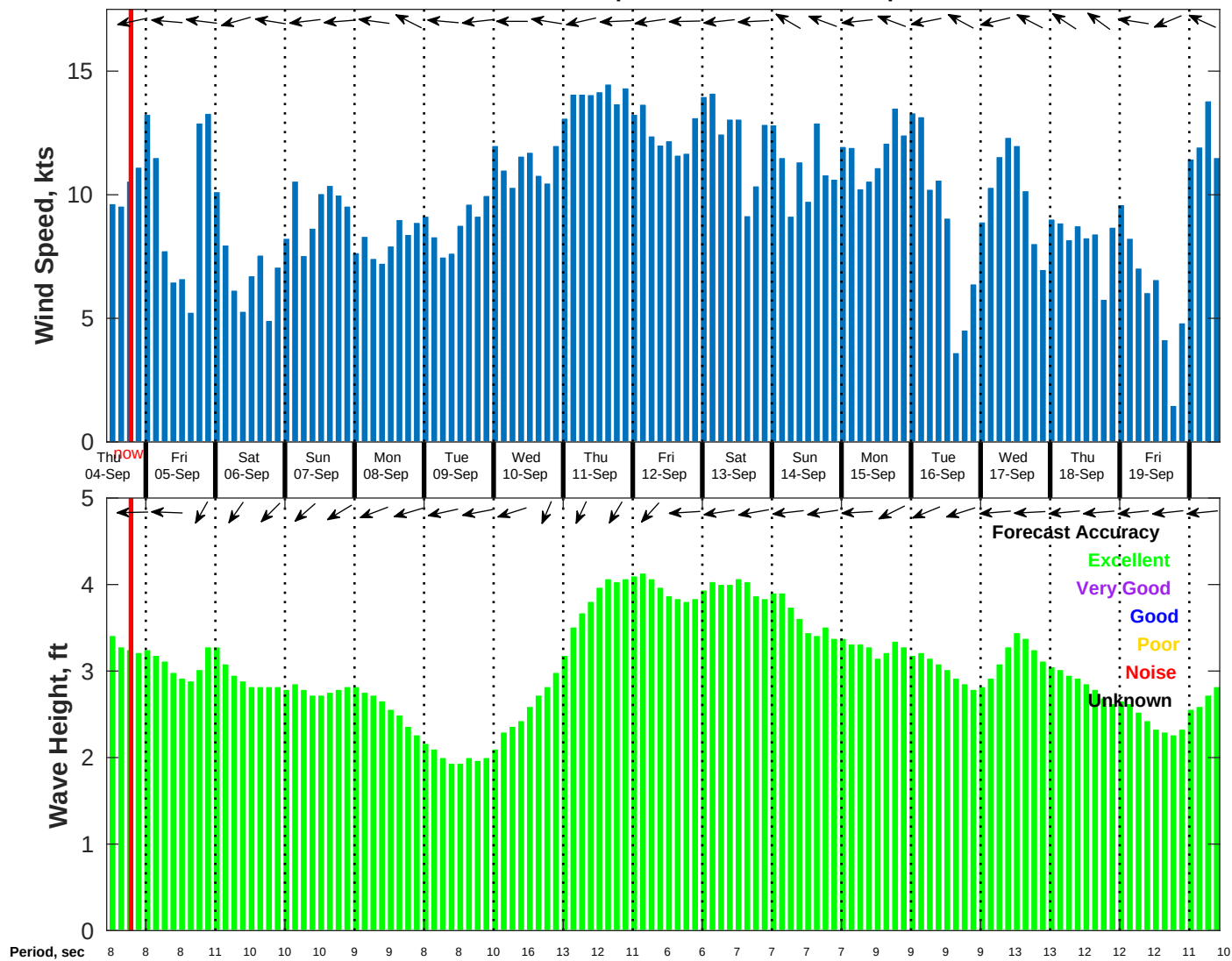
Wind & Wave Forecast for NDBC 52211 from 03-Sep-2025 11:00:00 to 19-Sep-2025 11:00:00
