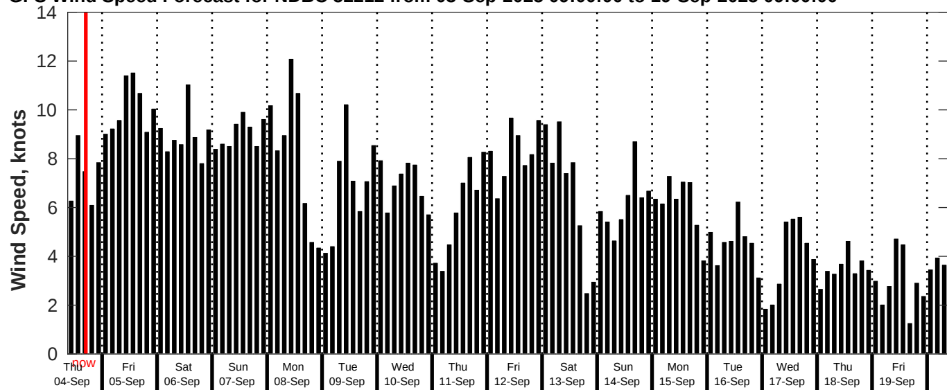
GFS Wind Speed Forecast for NDBC 52212 from 03-Sep-2025 09:00:00 to 19-Sep-2025 09:00:00
