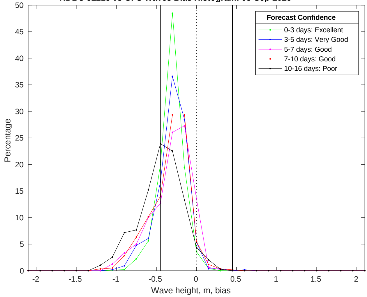
NDBC 52213 vs GFS Waves Bias Histogram: 03-Sep-2025
