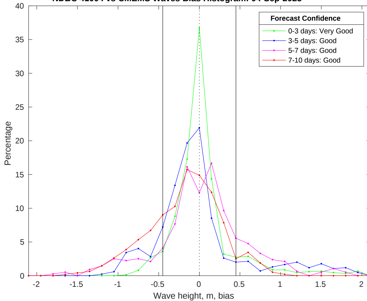
NDBC 41004 vs CMEMS Waves Bias Histogram: 04-Sep-2025
