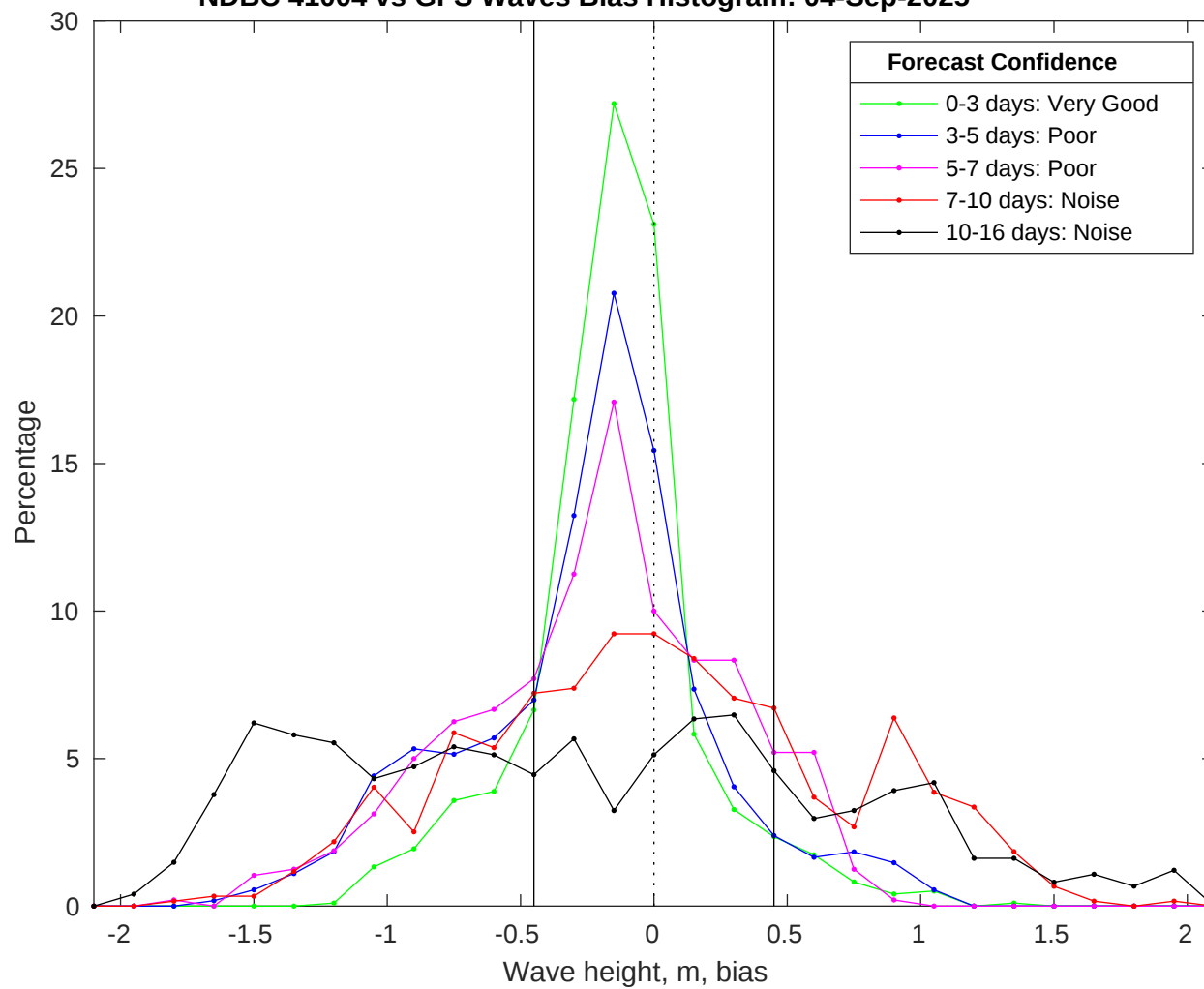
NDBC 41004 vs GFS Waves Bias Histogram: 04-Sep-2025
