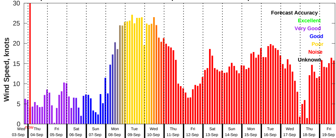
GFS Wind Speed Forecast for NDBC 41004 from 03-Sep-2025 19:00:00 to 19-Sep-2025 19:00:00
