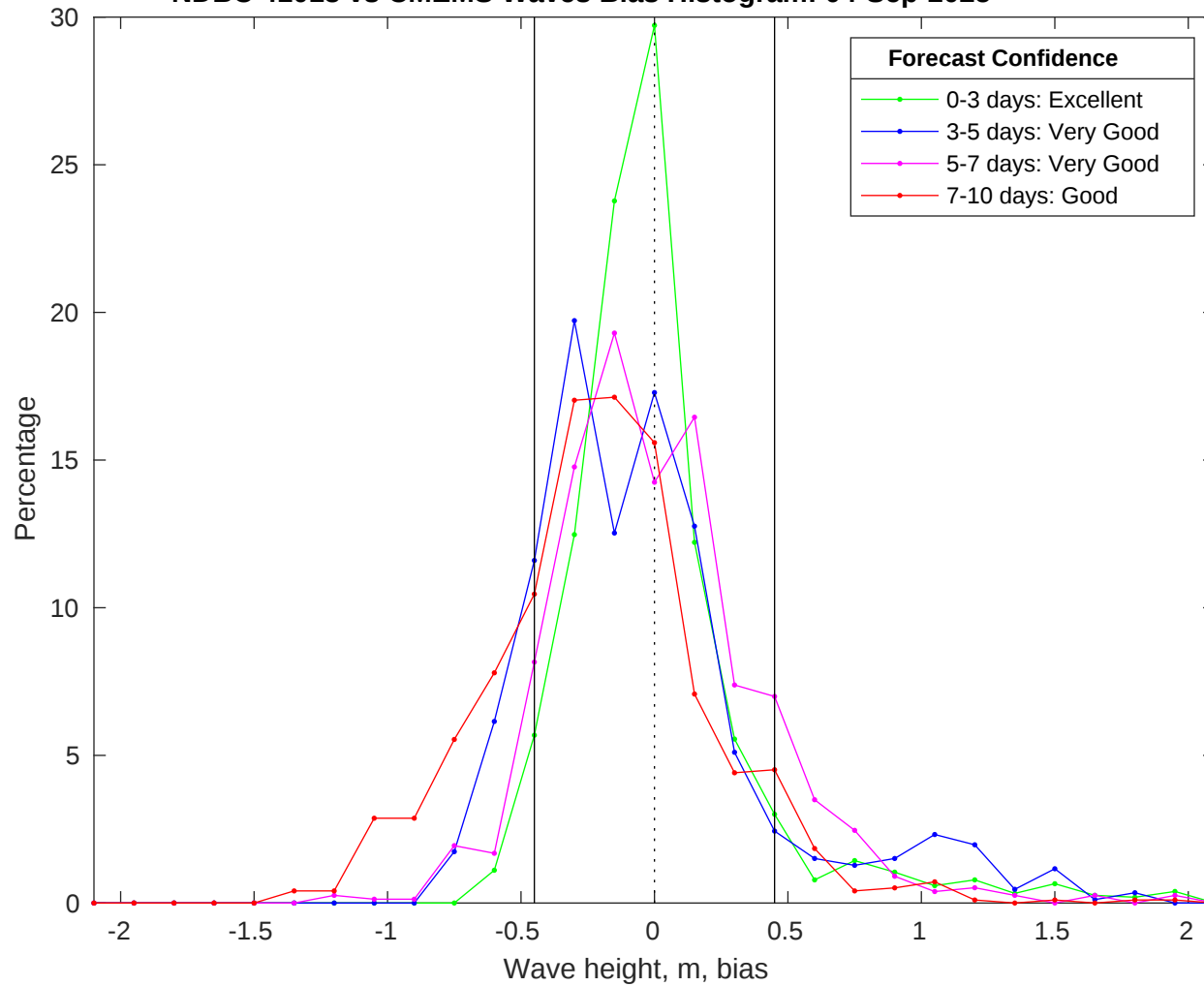
NDBC 41013 vs CMEMS Waves Bias Histogram: 04-Sep-2025
