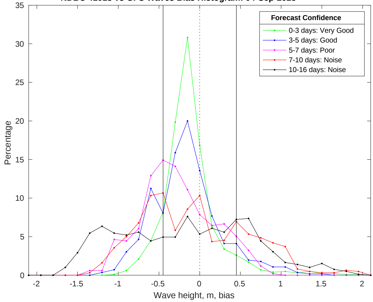
NDBC 41013 vs GFS Waves Bias Histogram: 04-Sep-2025
