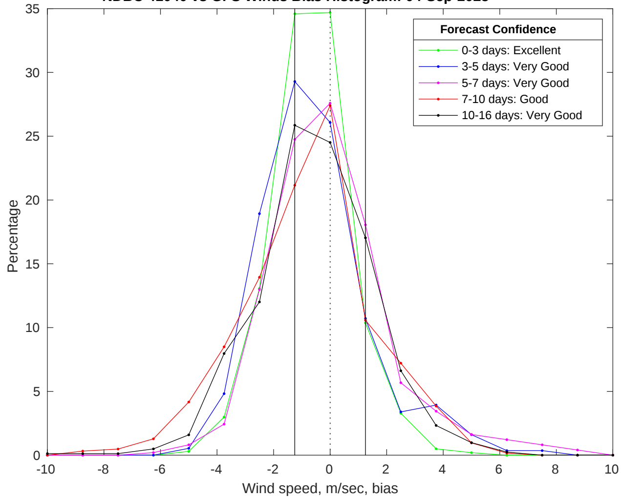
NDBC 41040 vs GFS Winds Bias Histogram: 04-Sep-2025
