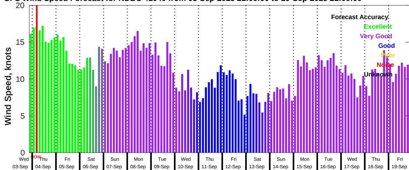
GFS Wind Speed Forecast for NDBC 41040 from 03-Sep-2025 21:00:00 to 19-Sep-2025 21:00:00
