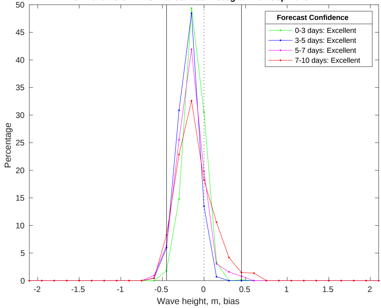
NDBC 42019 vs CMEMS Waves Bias Histogram: 04-Sep-2025
