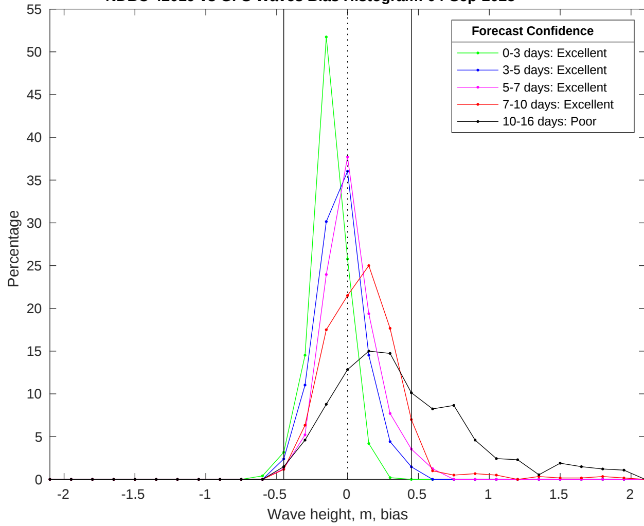
NDBC 42019 vs GFS Waves Bias Histogram: 04-Sep-2025
