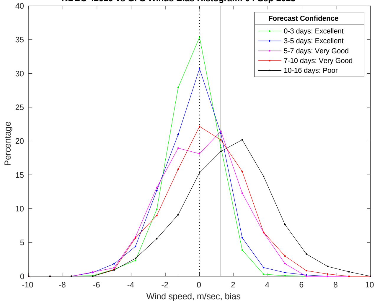
NDBC 42019 vs GFS Winds Bias Histogram: 04-Sep-2025
