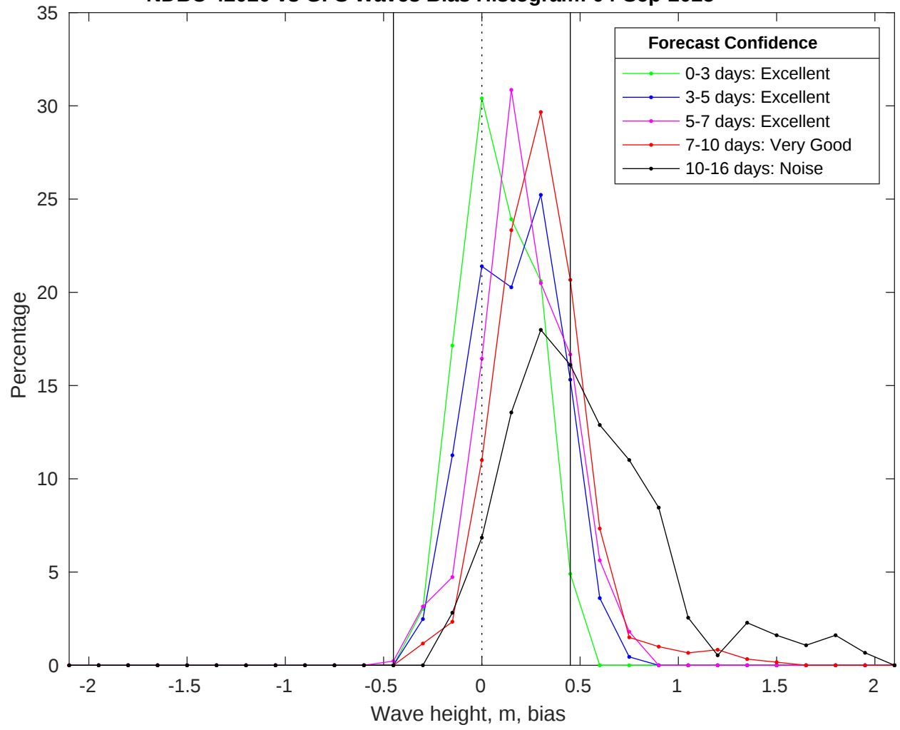
NDBC 42020 vs GFS Waves Bias Histogram: 04-Sep-2025
