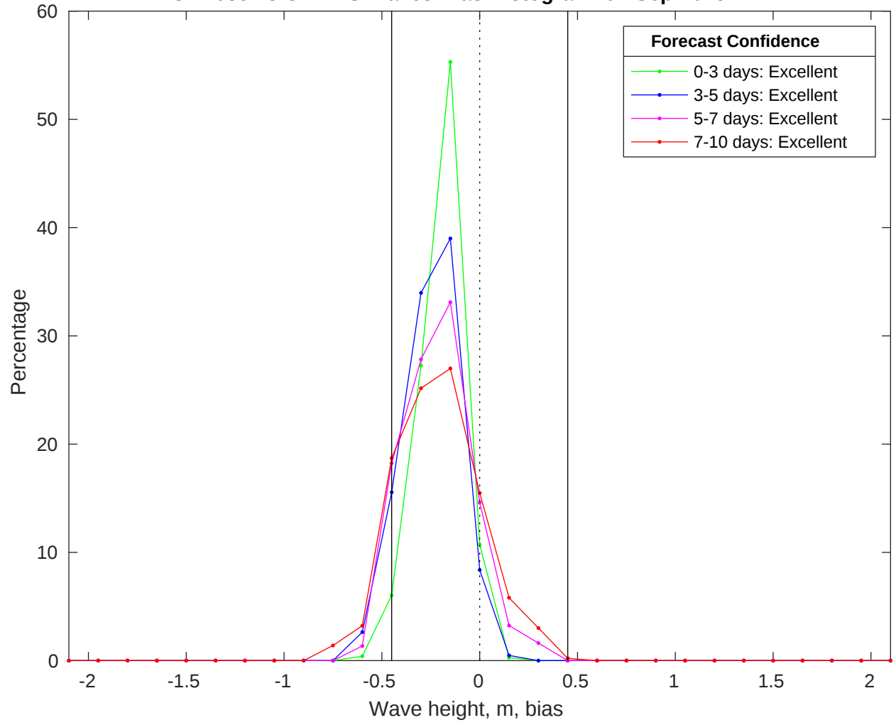
NDBC 42035 vs CMEMS Waves Bias Histogram: 04-Sep-2025
