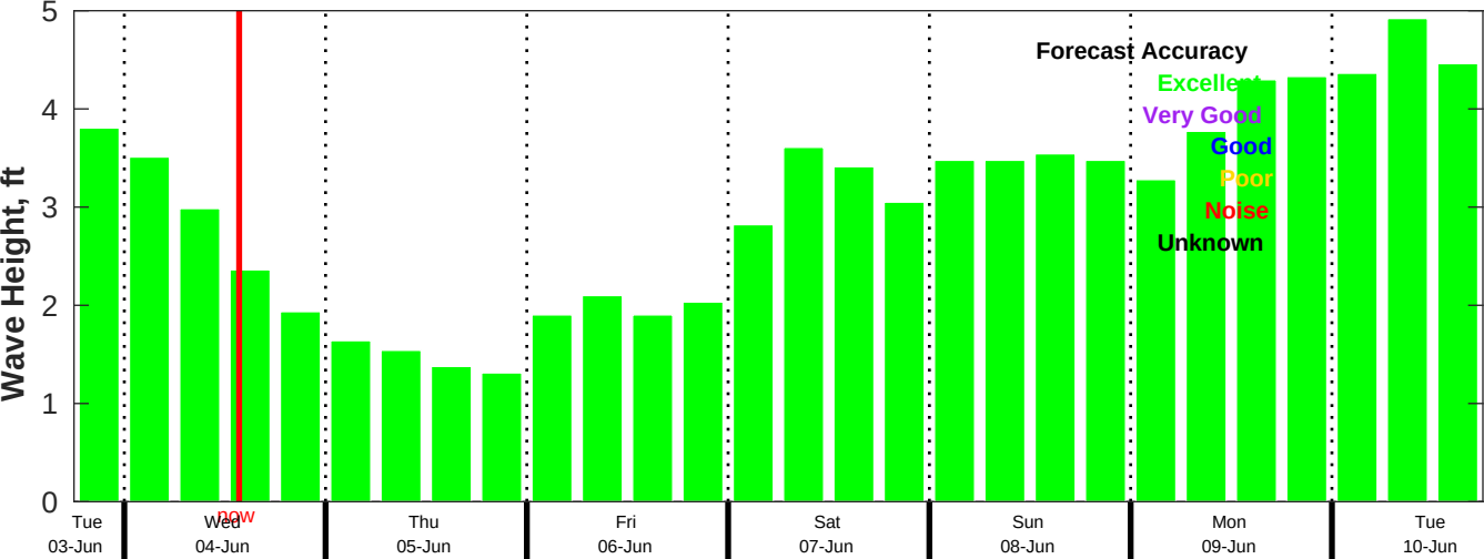
AUSWAV Wave Forecast for NDBC 42035 from 03-Jun-2025 18:00:00 to 10-Jun-2025 18:00:00
