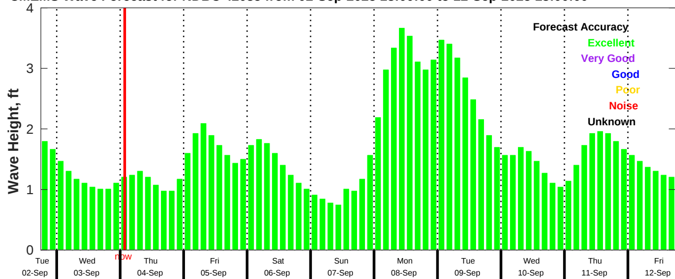
CMEMS Wave Forecast for NDBC 42035 from 02-Sep-2025 18:00:00 to 12-Sep-2025 18:00:00
