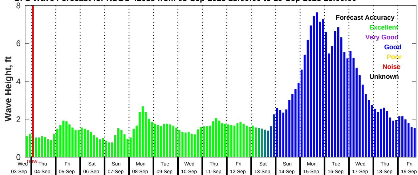
GFS Wave Forecast for NDBC 42035 from 03-Sep-2025 18:00:00 to 19-Sep-2025 18:00:00
