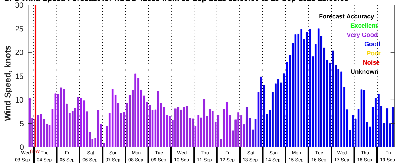
GFS Wind Speed Forecast for NDBC 42035 from 03-Sep-2025 18:00:00 to 19-Sep-2025 18:00:00
