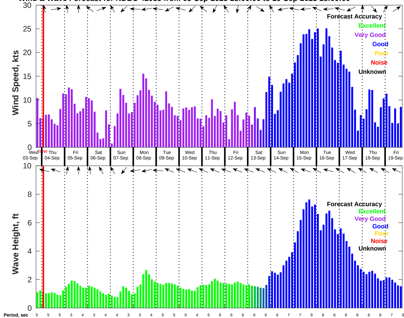
Wind & Wave Forecast for NDBC 42035 from 03-Sep-2025 18:00:00 to 19-Sep-2025 18:00:00
