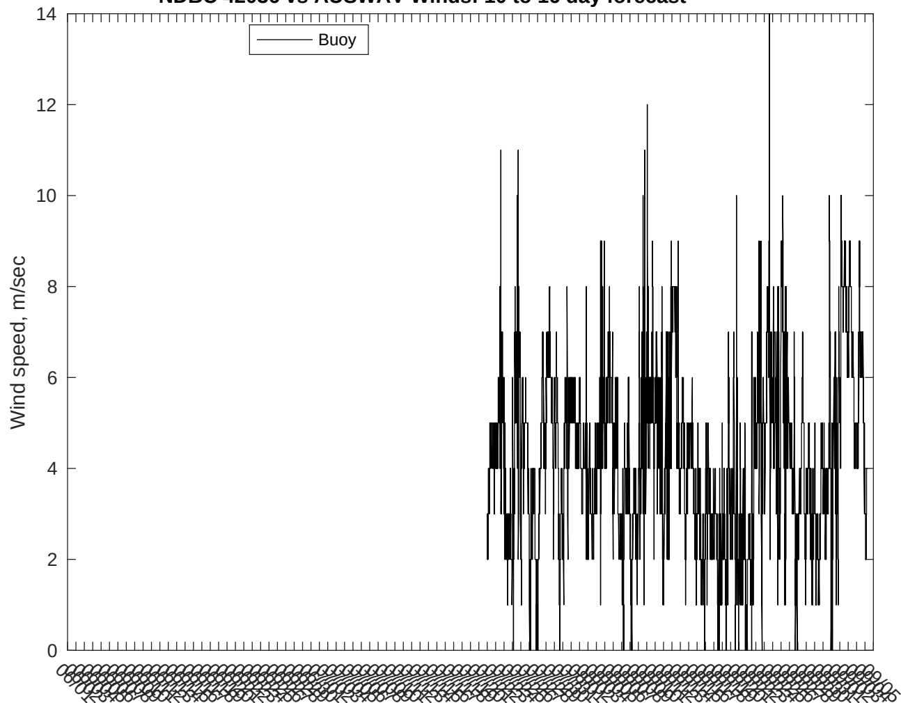
NDBC 42036 vs AUSWAV Winds: 10 to 16 day forecast
